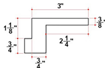
3" Zen Frame (3ZFL)
