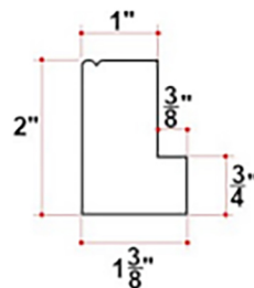
L Frame / K55
