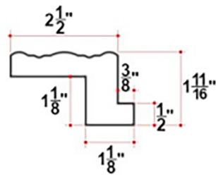
Fancy Trim / K45
