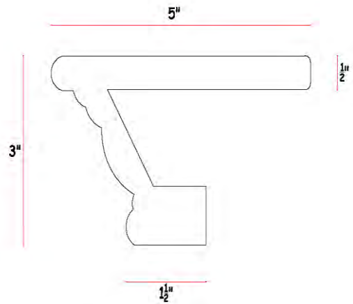
FC10 SILL CAP
