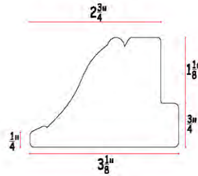
LD31 DECO L Z-FRAME
