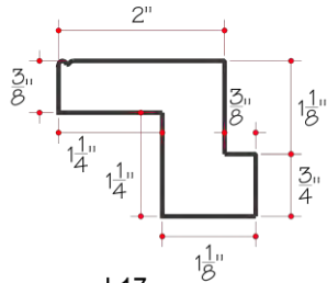
L17 Z-FRAME
