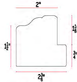
LD30 DECO L Z-FRAME
