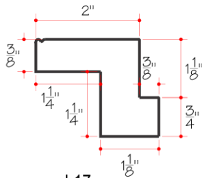
L17 Z-FRAME
